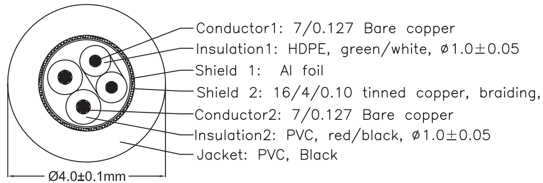
Cable Construction
